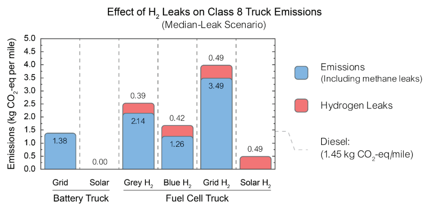
Figure VI-13. Comparative warming impact of Class 8 trucks for projected 2025 fuel efficiencies and grid emissions. Source: Argonne 2021 and EIA 2023c; leak estimates as for transit buses. 20-year global warming potentials used for hydrogen and upstream methane emissions.
