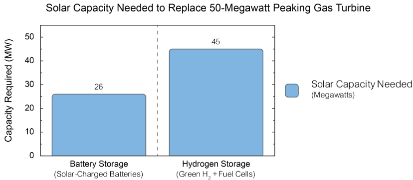
Figure VI-7: Solar generation capacity needed to replace a 50 MW peaking gas turbine with a solar + battery system or a green hydrogen + fuel cell system. Notes: (1) Gas turbine generation about 44,000 MW/year – about 10% capacity factor. (2) Assumed solar capacity factor: 22%
