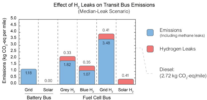
Figure VI-11: Effect of hydrogen leaks on transit bus warming impact. Sources: See notes to Figure VI-9 and Table VI-1 above.
