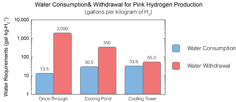
Figure IV-9: Comparison of water consumption and withdrawal requirements for nuclear electricity required for pink hydrogen production by cooling method; note the logarithmic scale on the vertical axis. Process water requirements of about 8 gallons per kilogram of hydrogen not shown. Source: Calculated using USGS 2019, Table 5.
