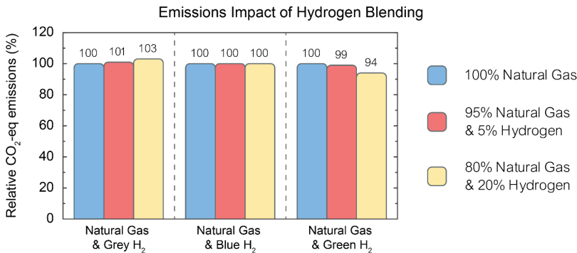
Figure VI-5: Relative greenhouse gas emissions for one million Btu of delivered energy for natural gas alone and natural gas blended with 5% and 20% hydrogen by volume – for grey, blue, and green hydrogen. Absolute emissions for natural gas = 96.3 kg CO 2 /million Btu. Source: IEER calculations, based on standard emission factors, and hydrogen production emissions as estimated in Chapter IV (based on the Argonne National Laboratory GREET model) and 2.7% natural gas leaks.
