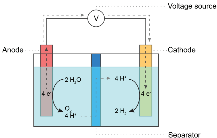
Figure IV-2: Schematic of an electrolyzer.
