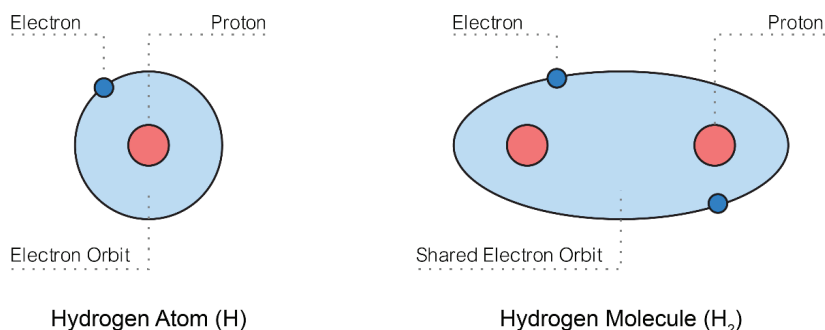
Figure II-1: Schematic representation of a hydrogen atom and molecule.
