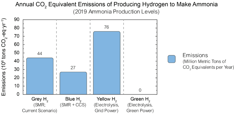
Figure VI-1: Methods of hydrogen production and the potential reduction of warming impact by transitioning from grey to blue or green hydrogen for ammonia production at the 2019 level of 14 million metric tons (3.0 million metric tons of hydrogen). GWP for methane 82.5. Hydrogen leaks assumed to be flared. Upstream emissions included. Capital investment indirect emissions not included. Methane leaks attributable to grid electricity generation system have been included. Source: IEER calculations based on 2.7% methane leaks, 20-year methane warming potential and Argonne 2022 for other emission estimates (see Figure IV-4 above).
