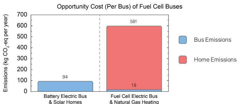
Figure VI-12: Comparison of two options for using solar energy – an FCEB or converting natural gas heated homes. Notes: National average natural gas use per home using natural gas = 81 million Btu. 335 Number of homes using natural gas heating = 59.2 million. 336
