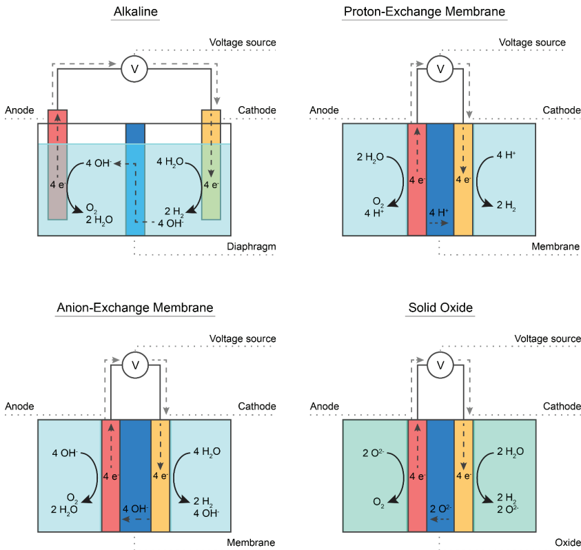
Figure IV-3: Schematic depictions of 4 common electrolyzer types.
