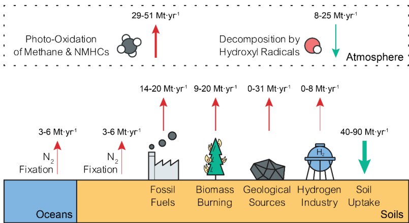
Figure III-1: Sources and sinks of hydrogen, in million metric tons per year. CH 4 is methane; NMHCs are non-methane hydrocarbons. Mt = million metric tons. Source: Based on Figure 1 in Arrigoni and Bravo-Diaz 2022, and adapted for this report under Creative Commons Copyright.
