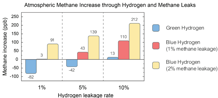
Figure S-2: Net change in global methane concentrations at three hydrogen leak rates and two methane leak rates when hydrogen displaces about ~15% of global fossil fuel use.
