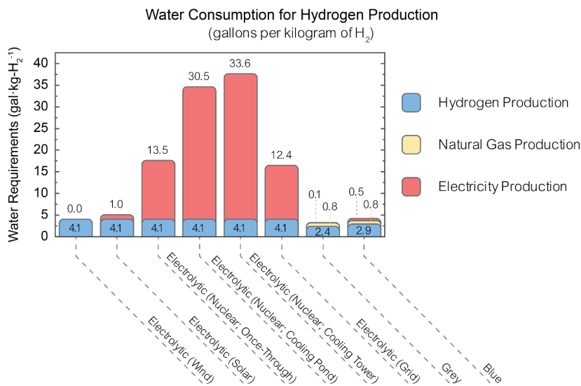
Figure IV-8: Water consumption for various methods of hydrogen production. Steam methane reforming without CCS (“grey” hydrogen) is the current dominant technology. Values rounded to the nearest tenth of a gallon. The numbers at the tops of the bars represent the water consumption for the electricity portion alone. The total water use should be read off from the axis at the left of the chart.
