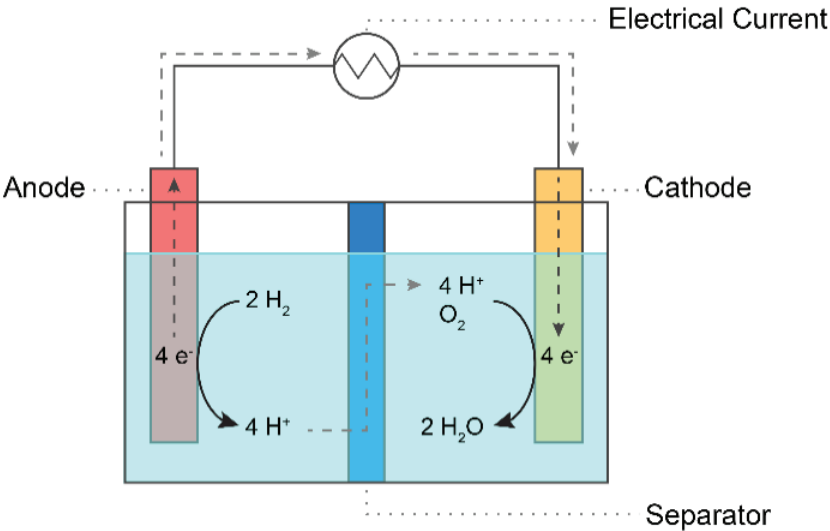
Figure VI-8: Schematic depiction of a fuel cell.
